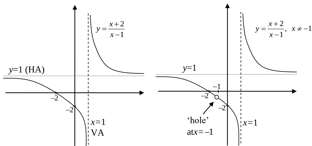
Fig 2.3 (A) f(x) = \frac{x+2}{x-1}
